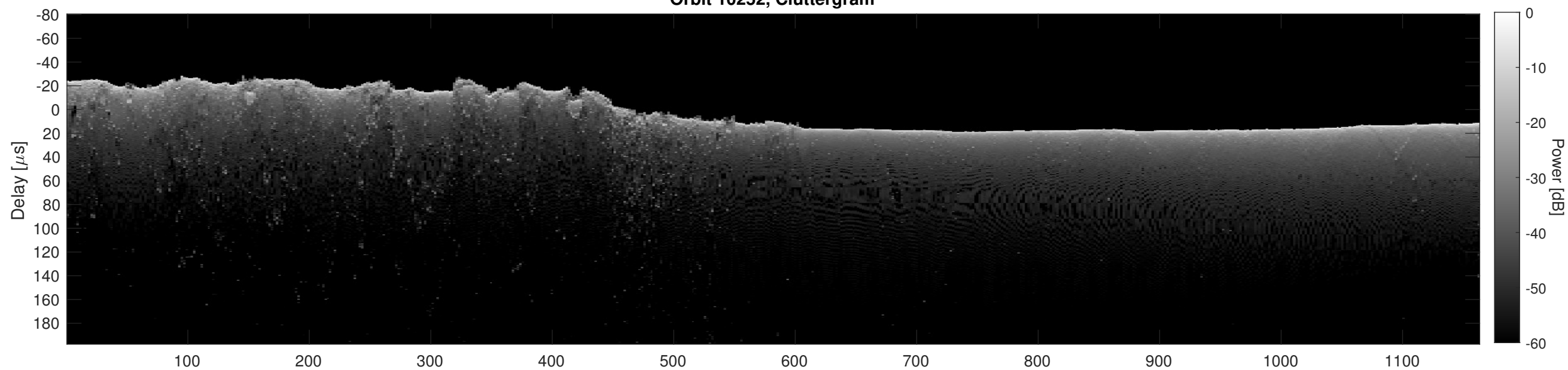
Orbit 10252, Cluttergram
