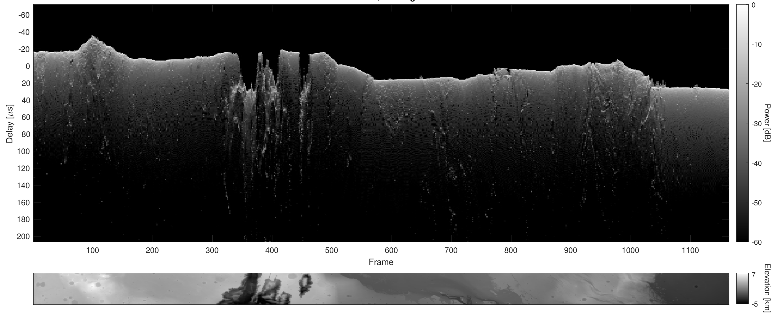
Orbit 10254, Cluttergram
