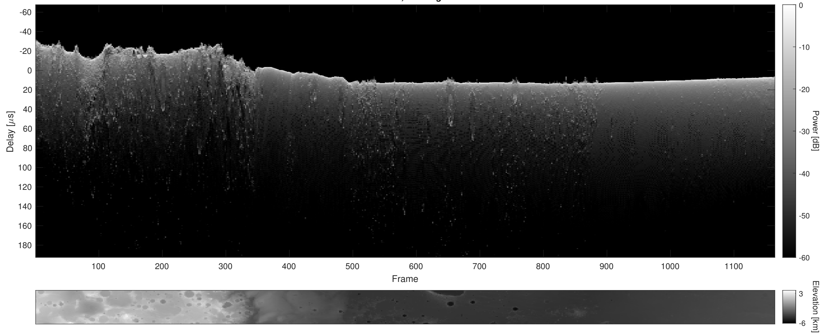
Orbit 10255, Cluttergram
