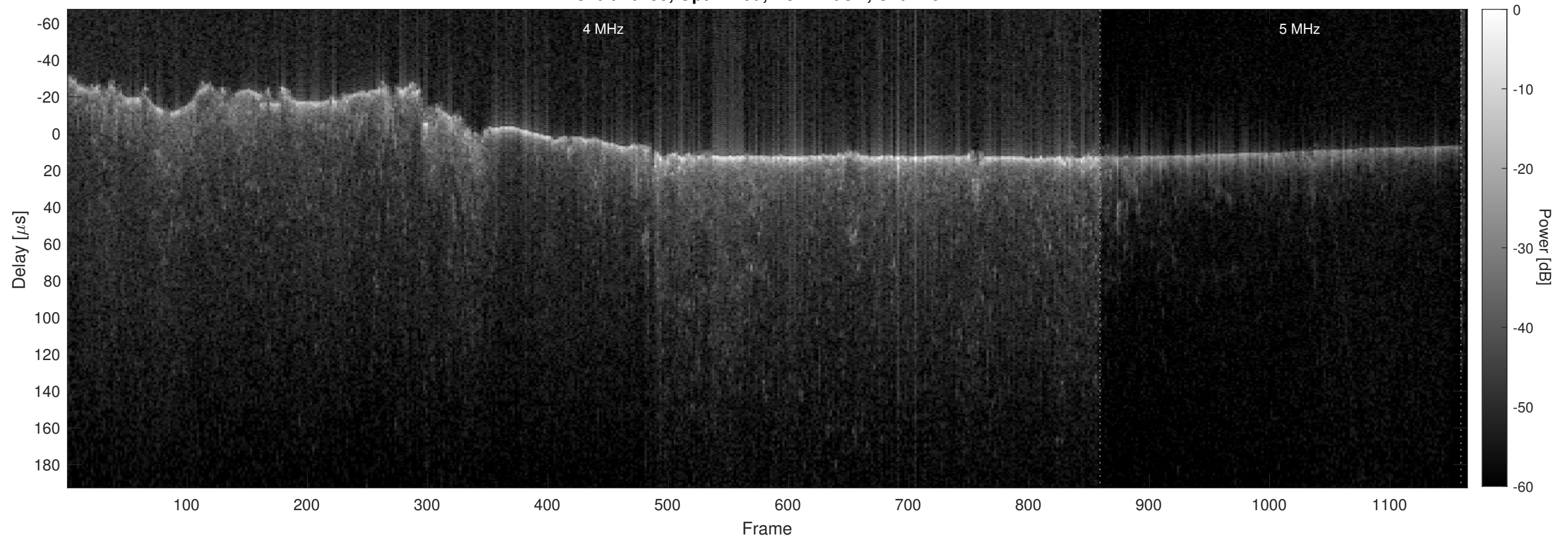
Orbit 10255, Optimized, No Window, Channel 2
