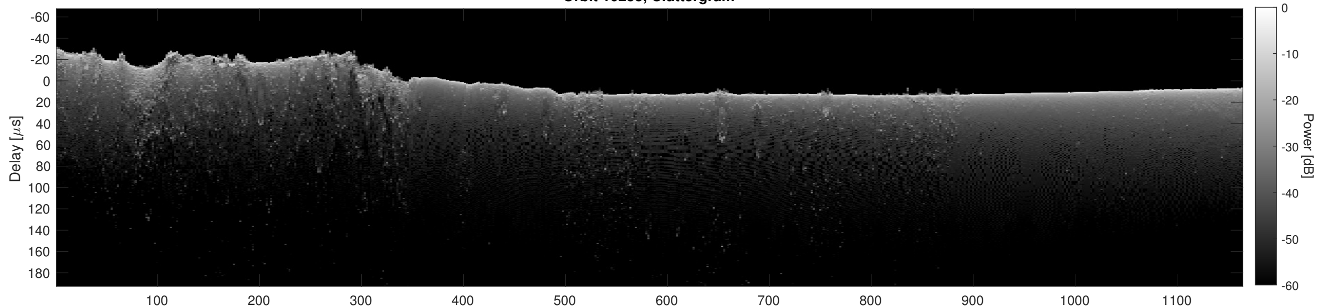
Orbit 10255, Cluttergram
