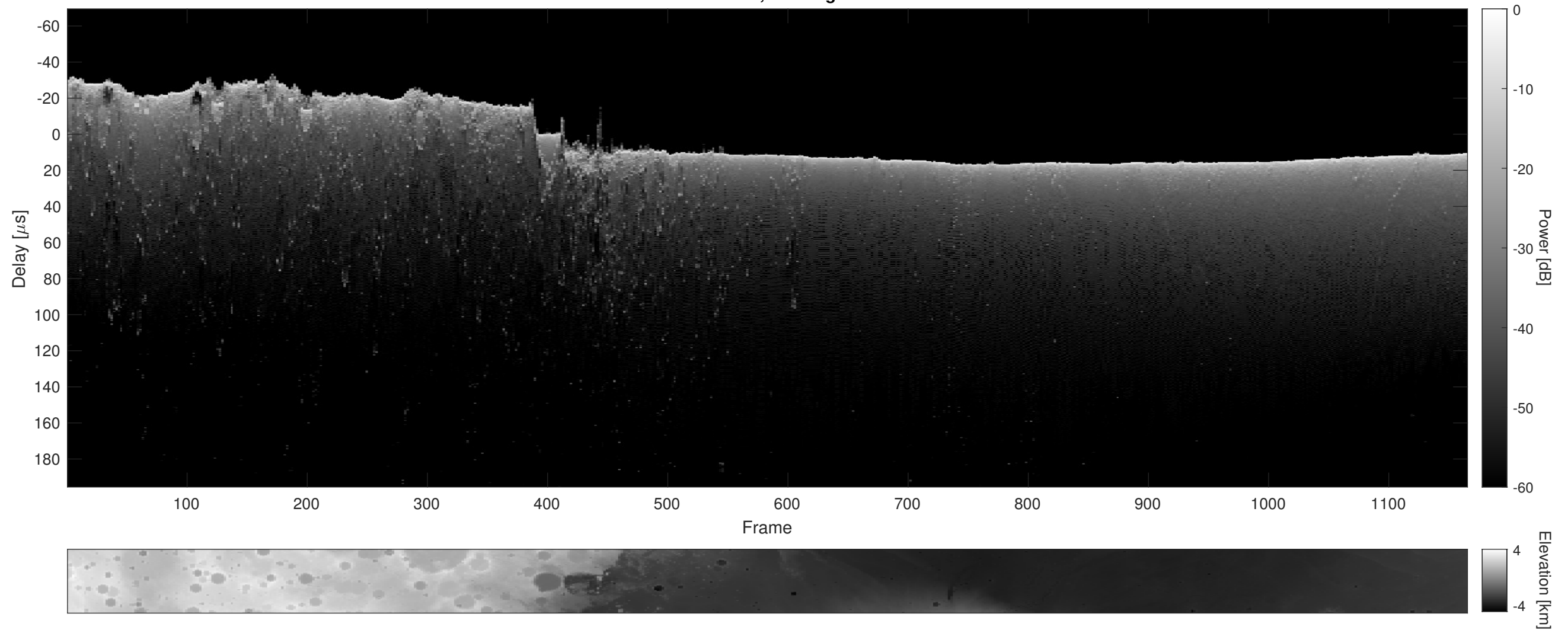
Orbit 10259, Cluttergram
