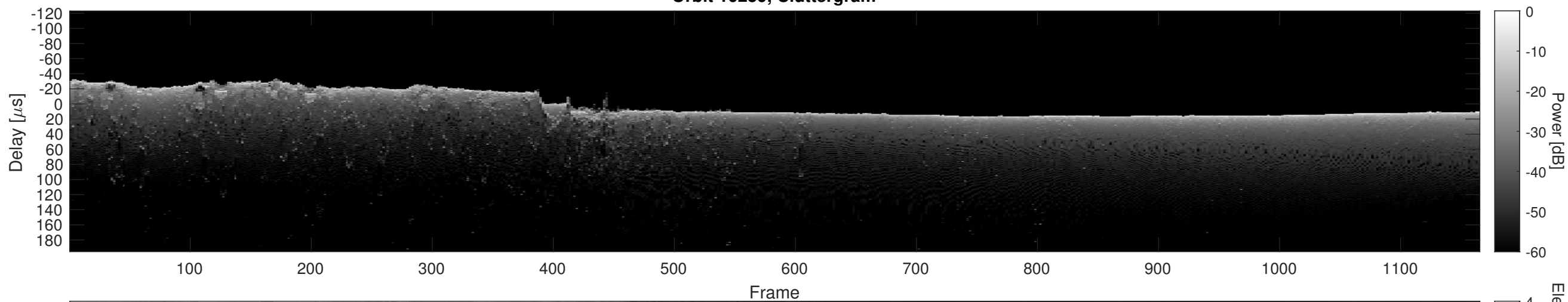
Orbit 10259, Cluttergram
