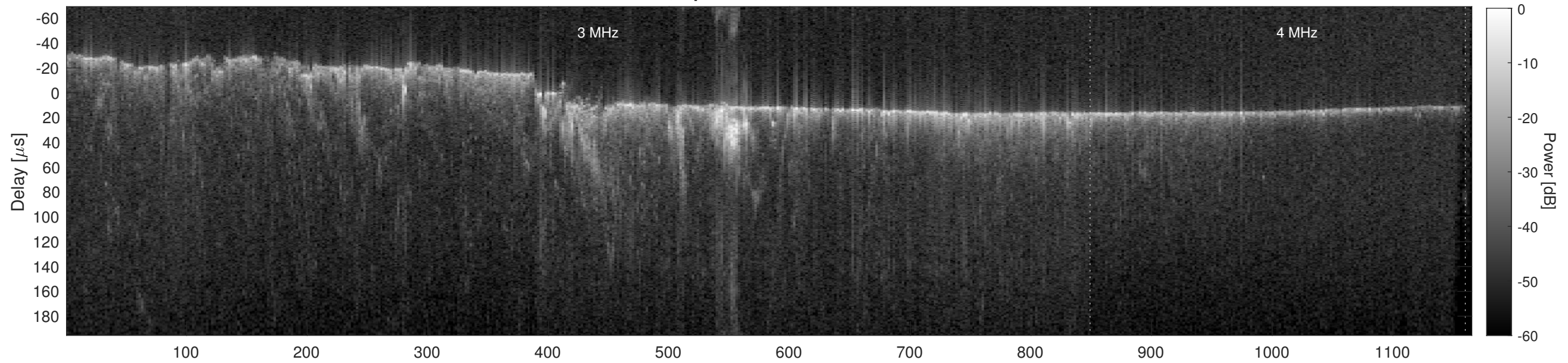
Orbit 10259, Cluttergram
