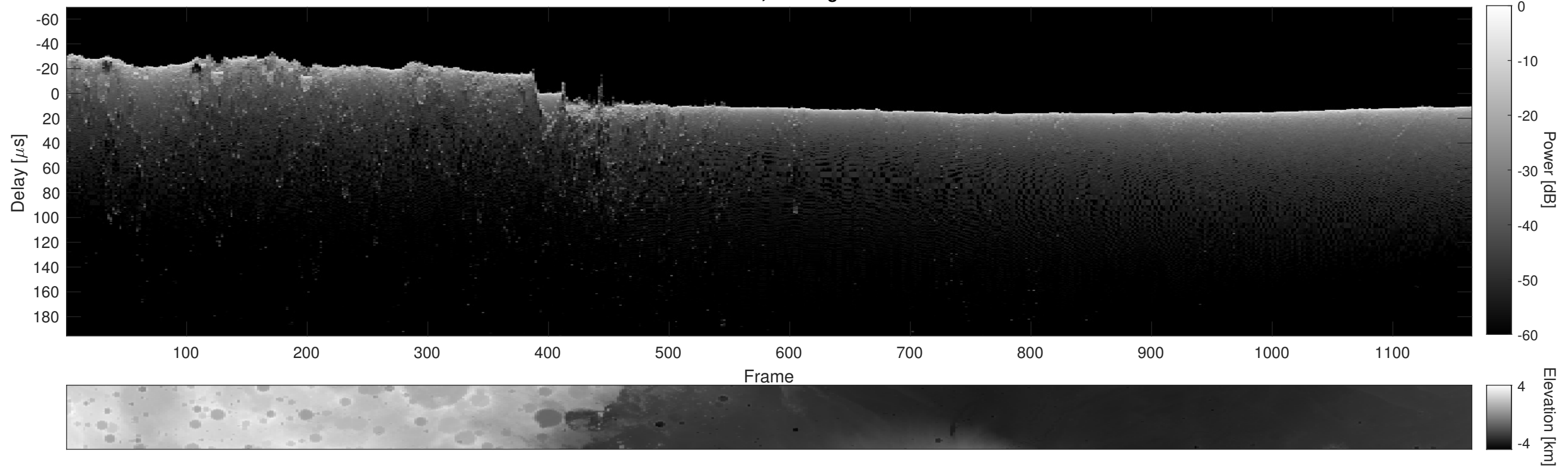
Orbit 10259, Cluttergram
