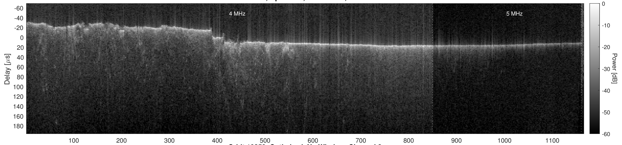
Orbit 10259, Optimized, No Window, Channel 2
