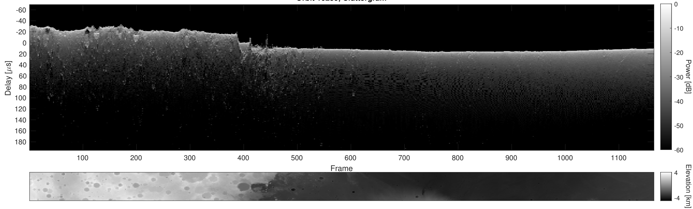
Orbit 10259, Cluttergram
