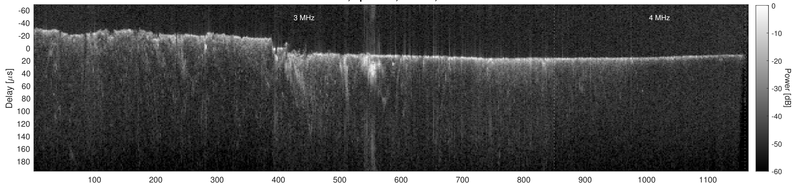
Orbit 10259, Cluttergram
