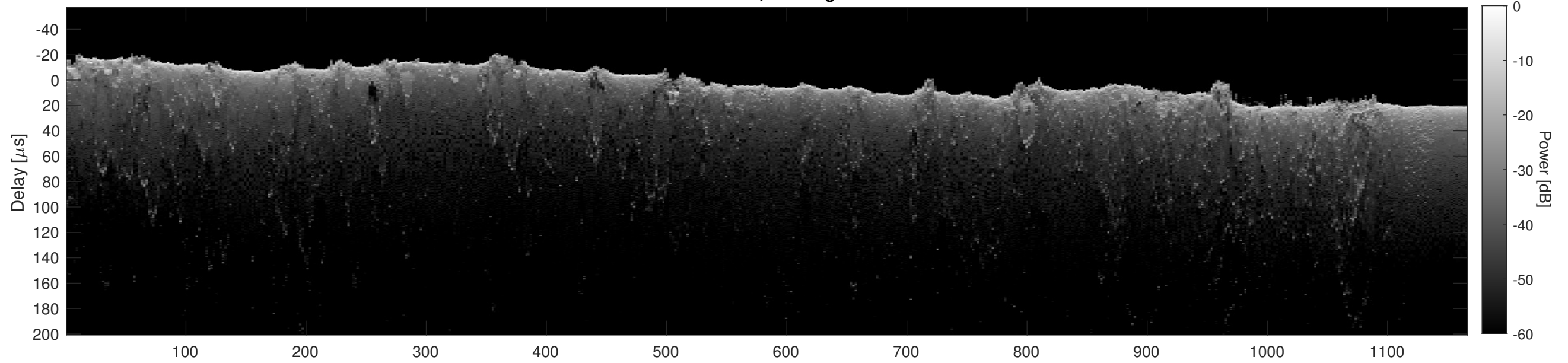
Orbit 10260, Cluttergram
