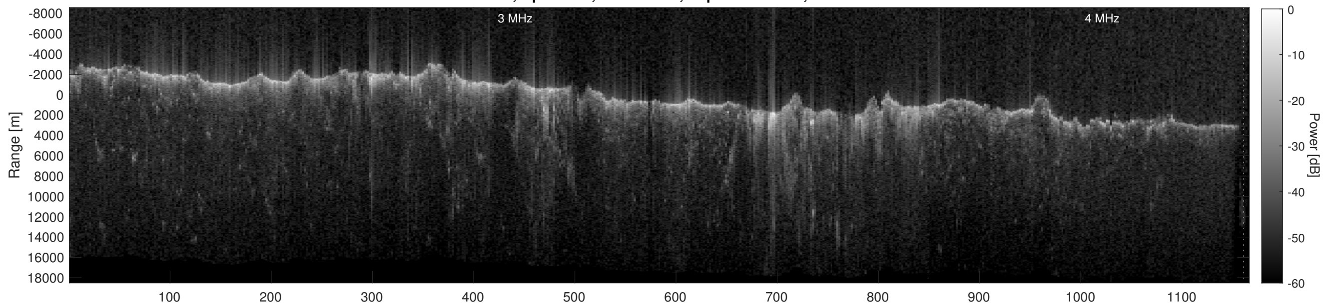
Orbit 10260, Depth-Corrected Cluttergram
