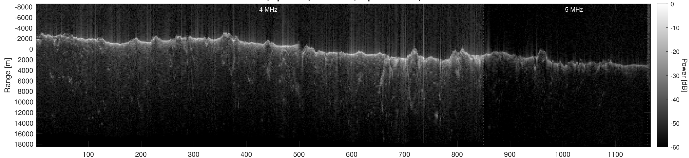
Orbit 10260, Optimized, No Window, Depth-Corrected, Channel 2
