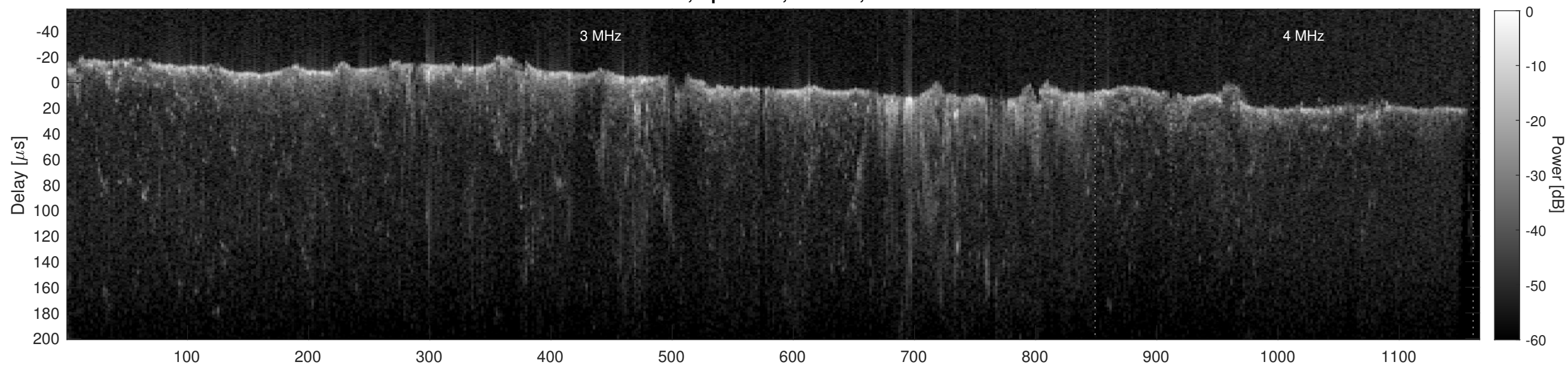
Orbit 10260, Cluttergram
