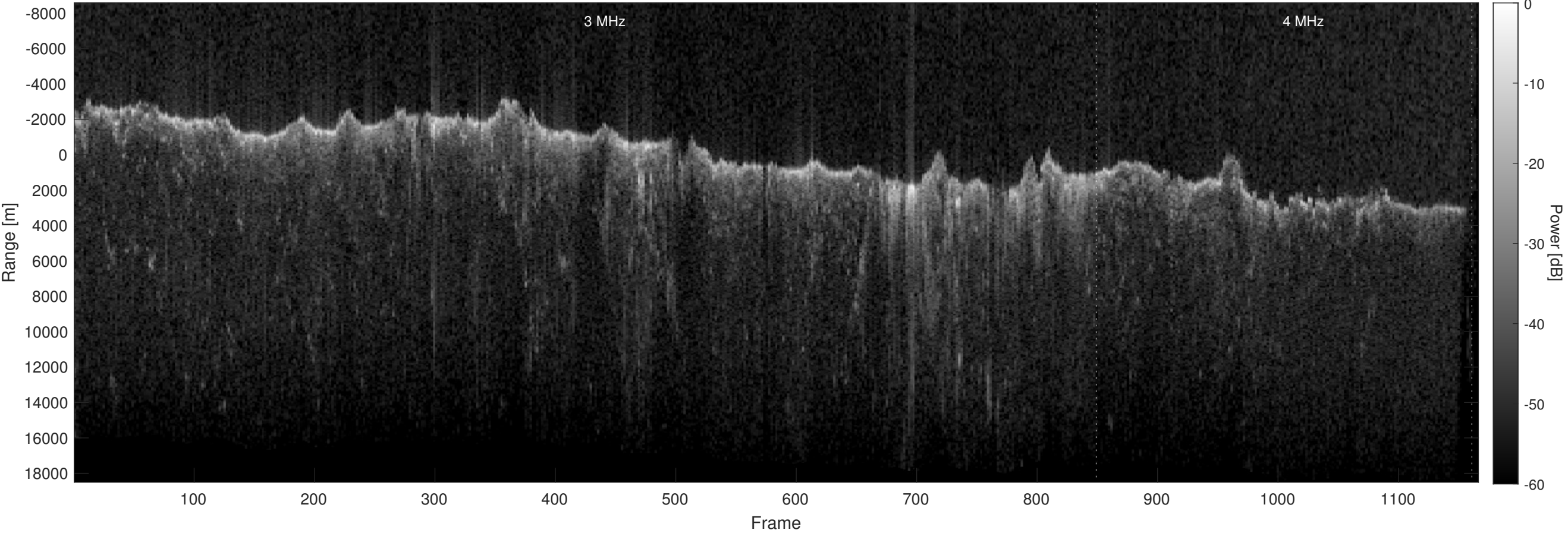
Orbit 10260, Optimized, Window, Depth-Corrected, Channel 2
