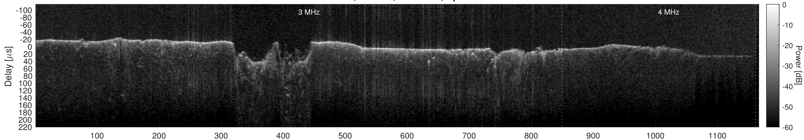
Orbit 10261, Cluttergram
