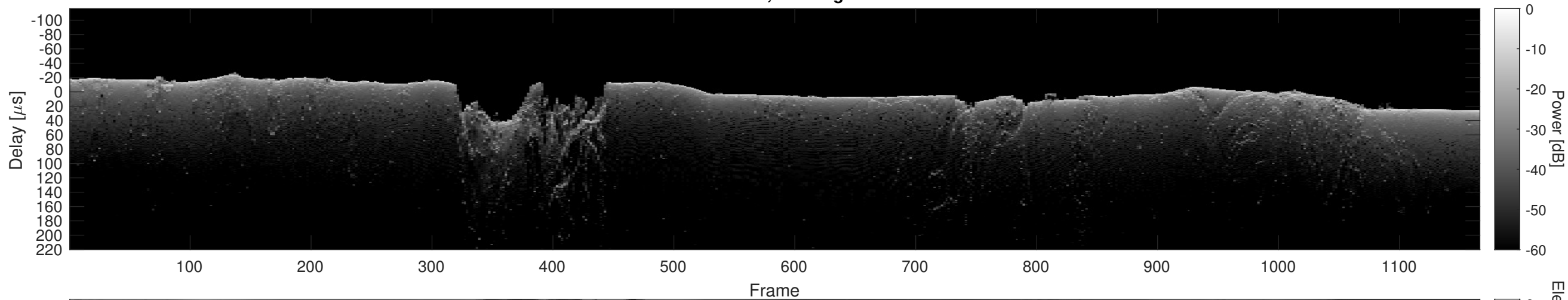
Orbit 10261, Cluttergram
