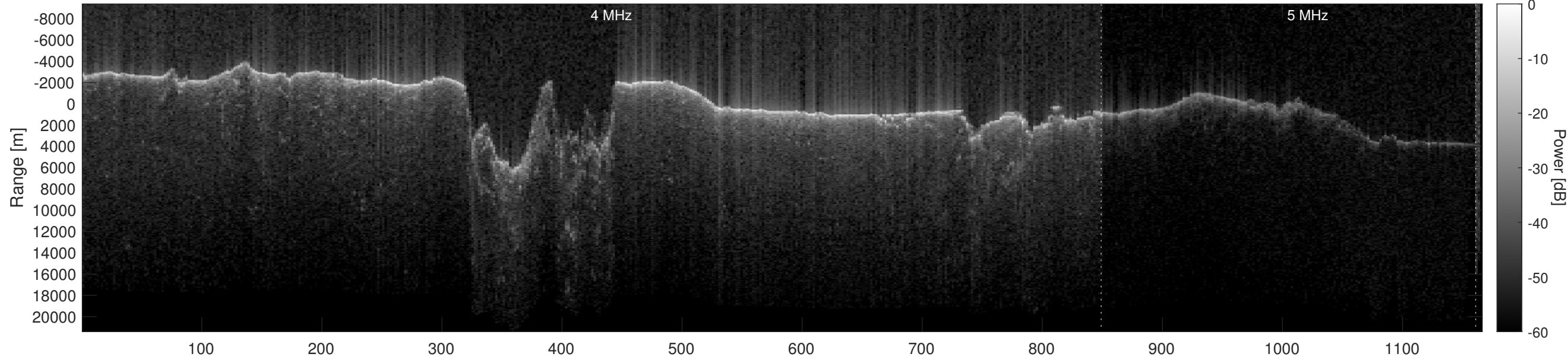
Orbit 10261, Optimized, No Window, Depth-Corrected, Channel 2
