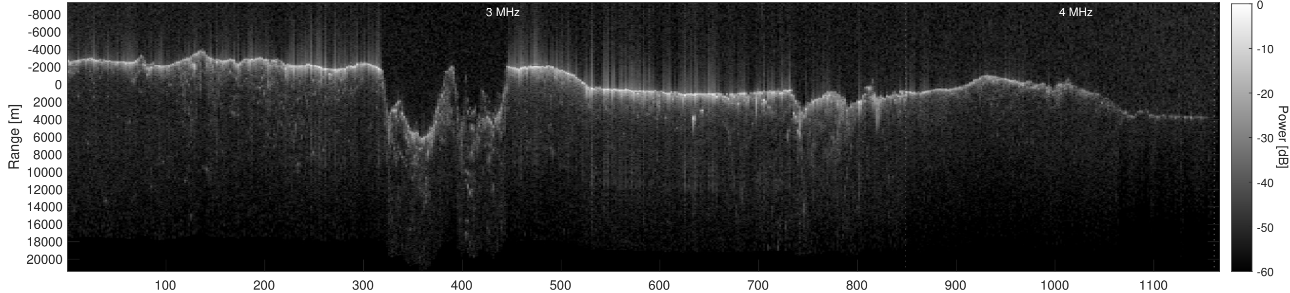
Orbit 10261, Depth-Corrected Cluttergram
