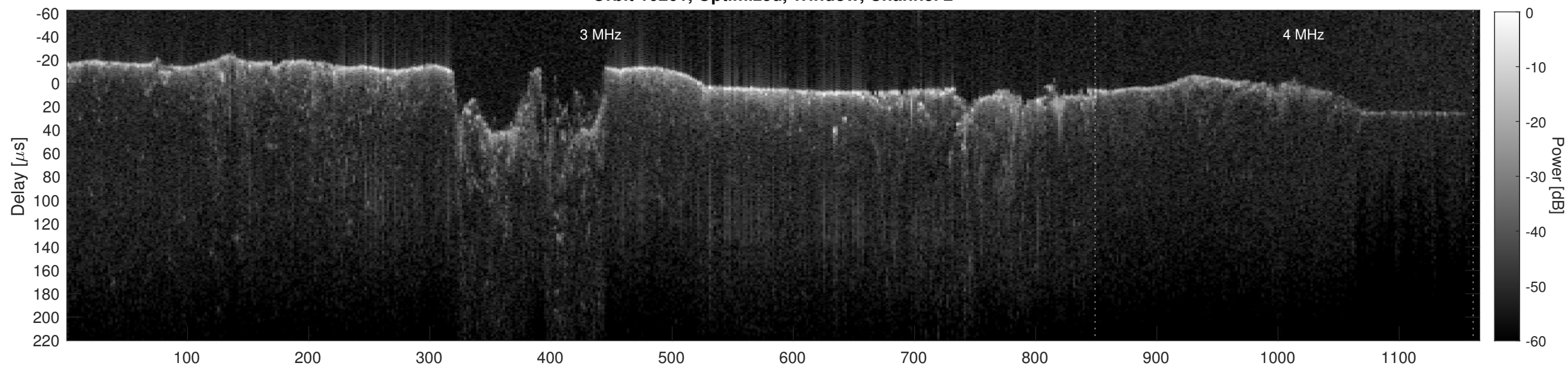
Orbit 10261, Cluttergram
