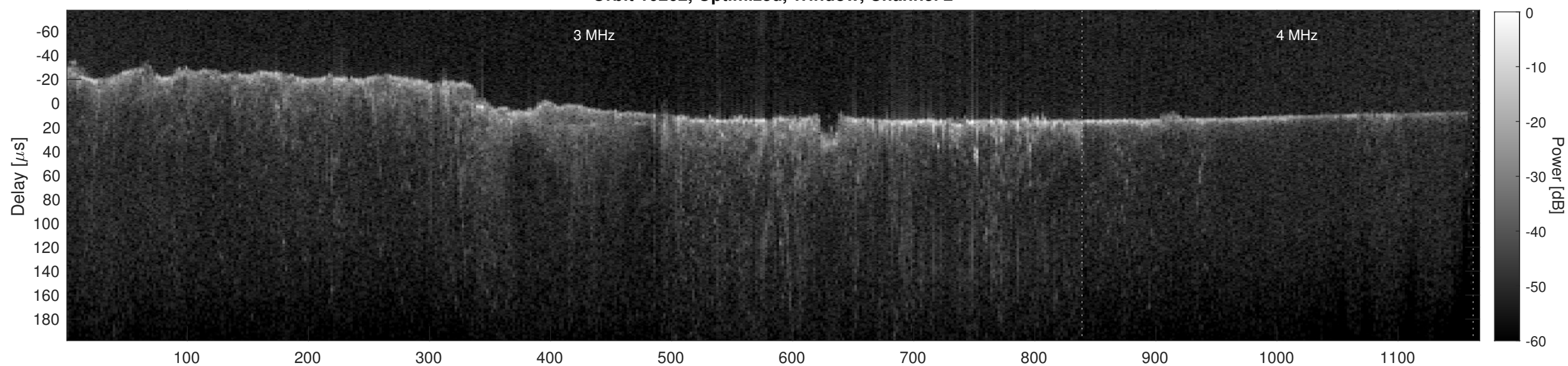
Orbit 10262, Cluttergram
