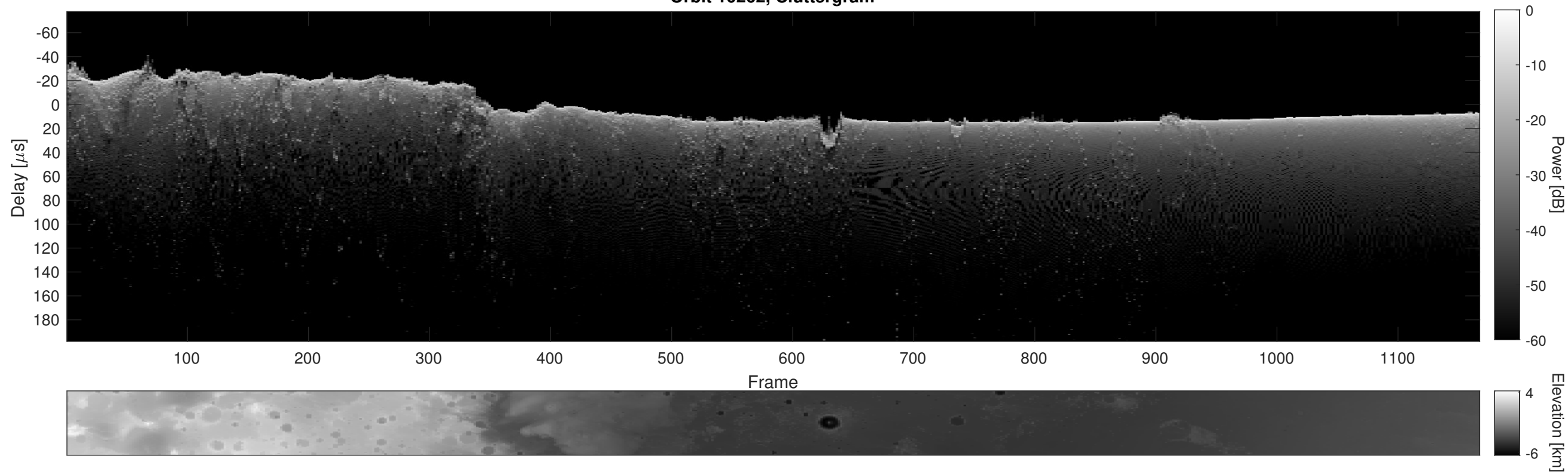
Orbit 10262, Cluttergram
