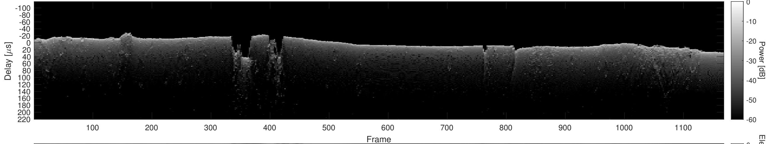
Orbit 10268, Cluttergram
