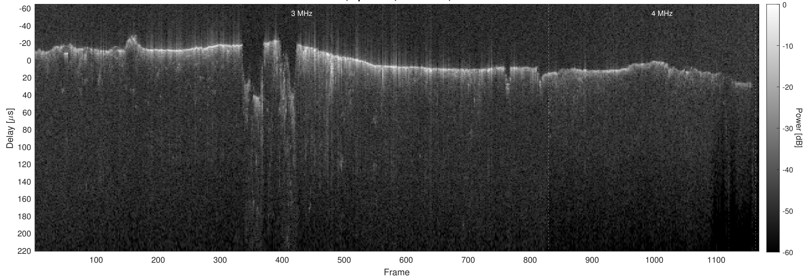
Orbit 10268, Optimized, No Window, Channel 2
