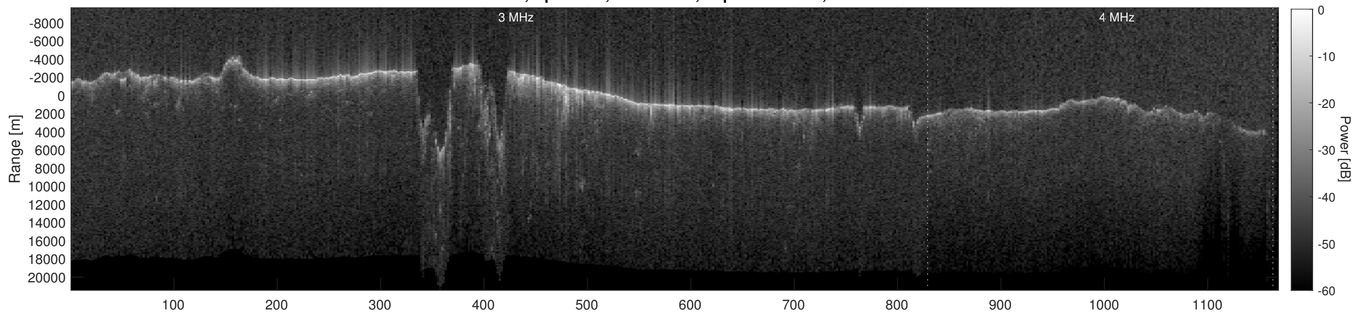
Orbit 10268, Depth-Corrected Cluttergram
