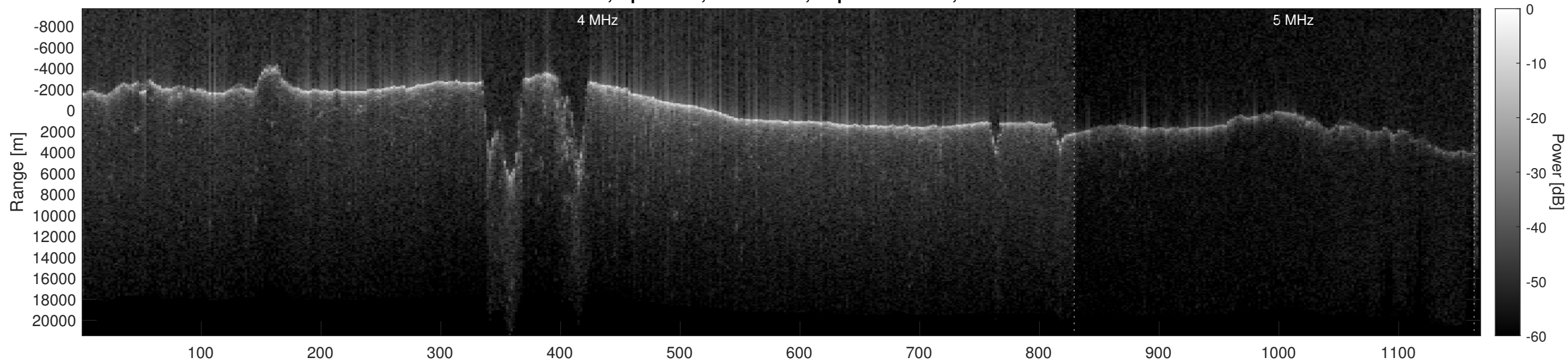
Orbit 10268, Optimized, No Window, Depth-Corrected, Channel 2
