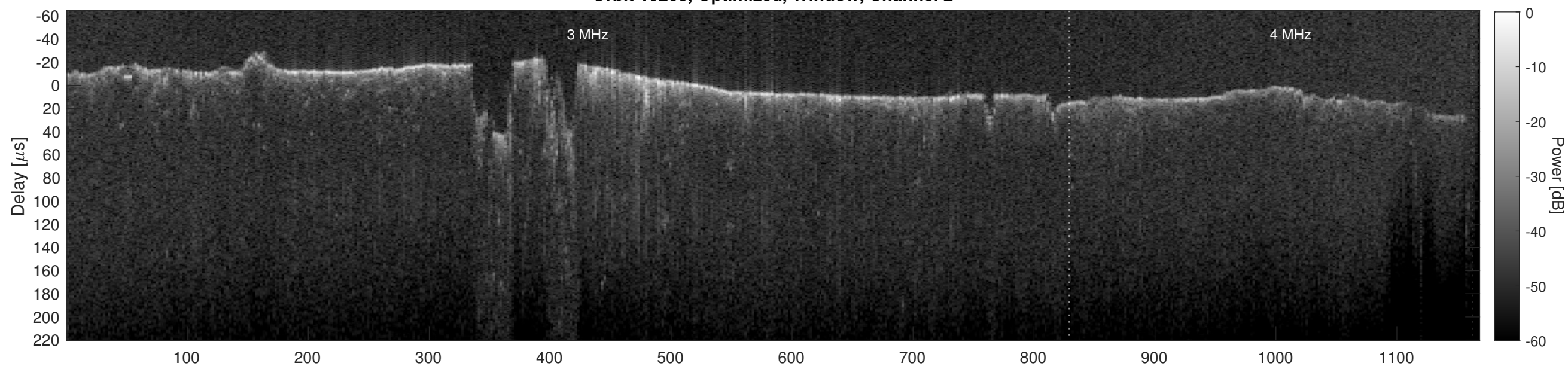
Orbit 10268, Cluttergram
