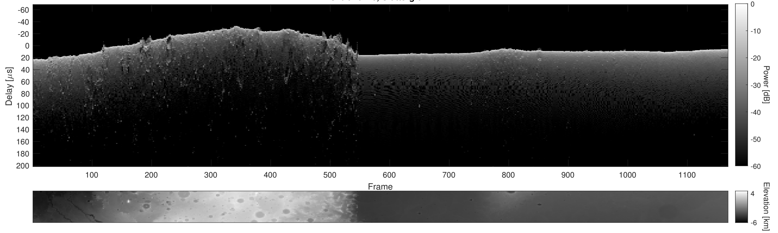
Orbit 10270, Cluttergram
