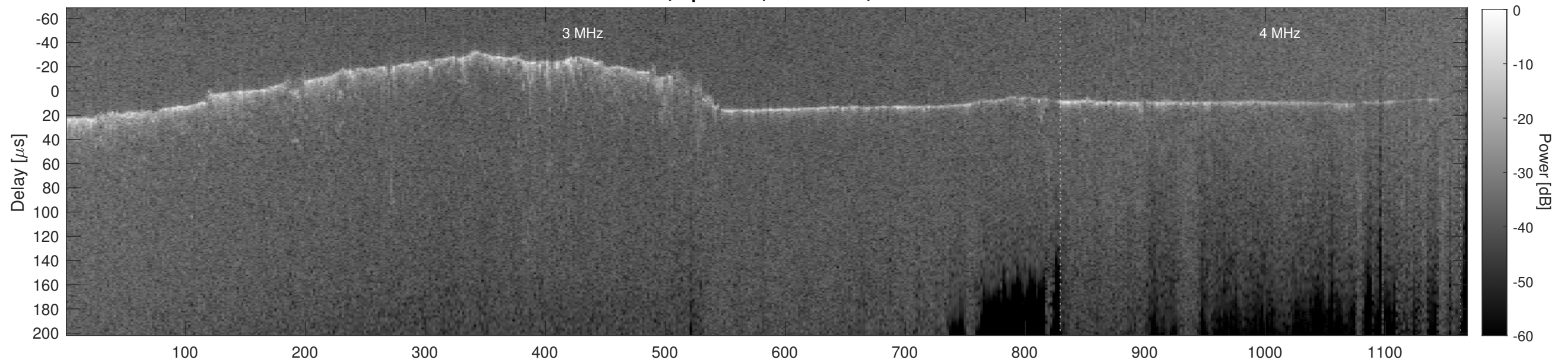
Orbit 10270, Cluttergram
