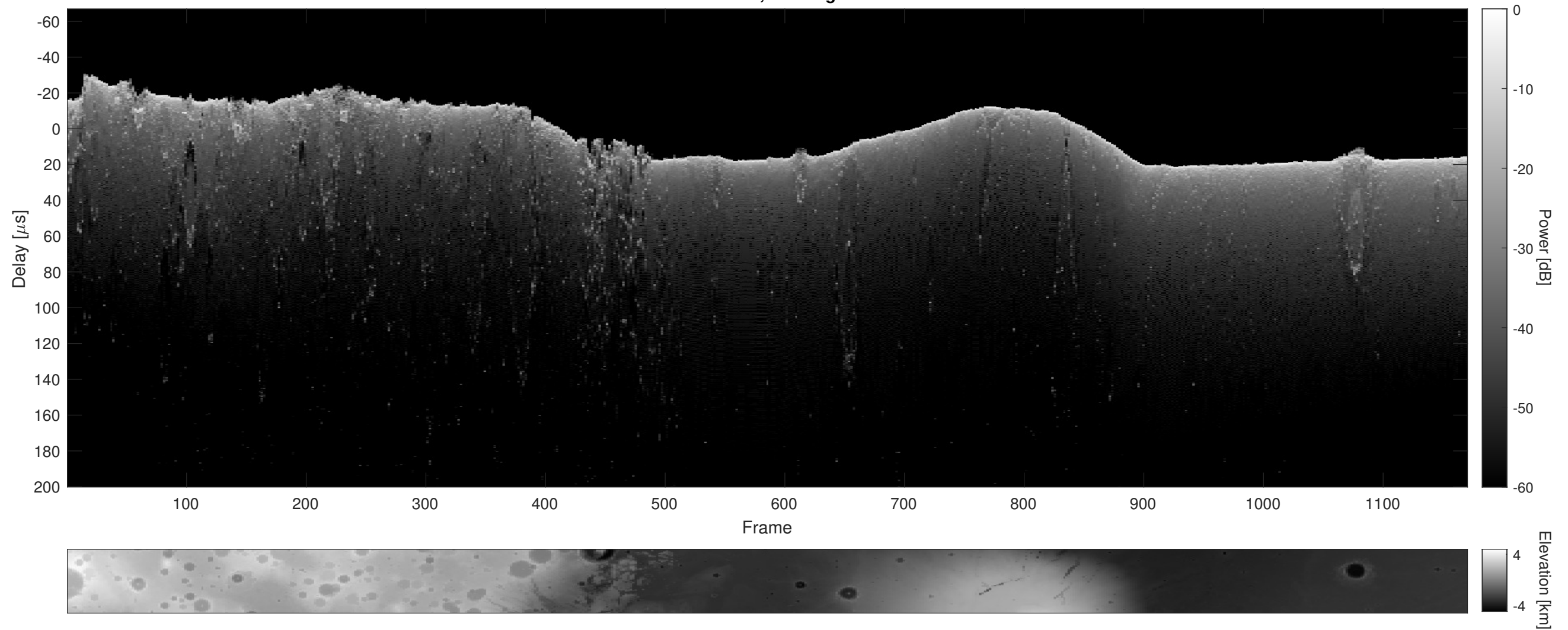
Orbit 10273, Cluttergram
