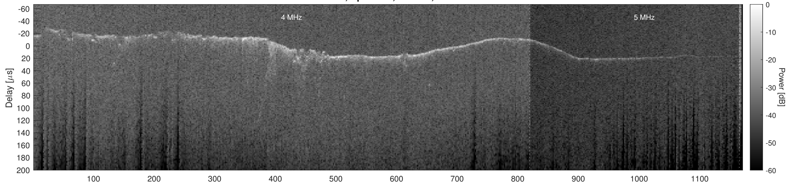
Orbit 10273, Optimized, Window, Channel 2
