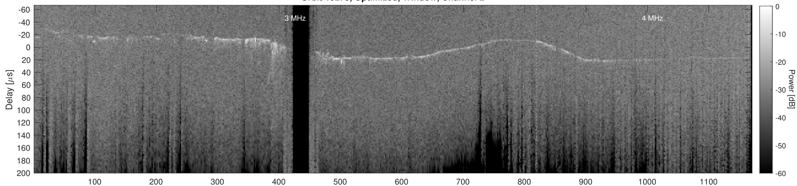
Orbit 10273, Cluttergram
