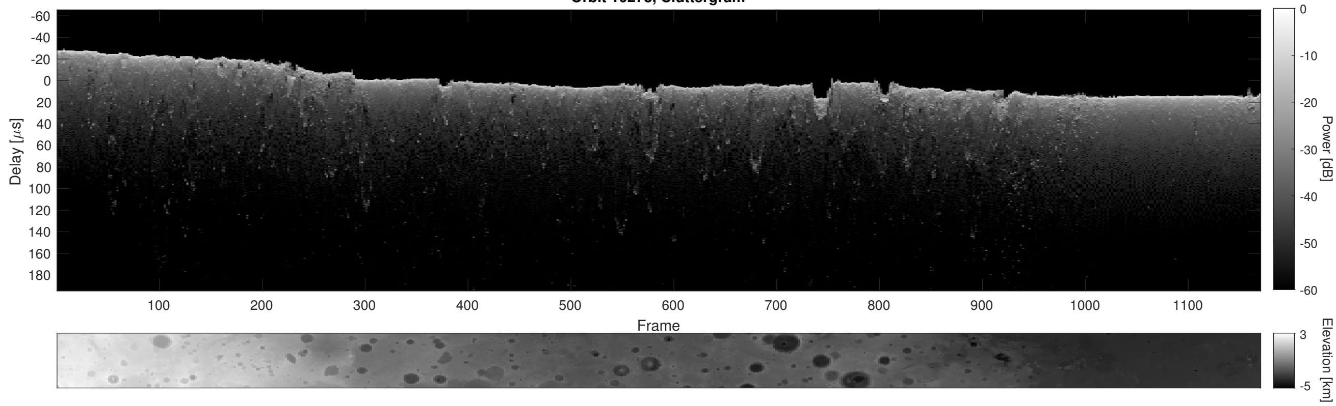
Orbit 10278, Cluttergram
