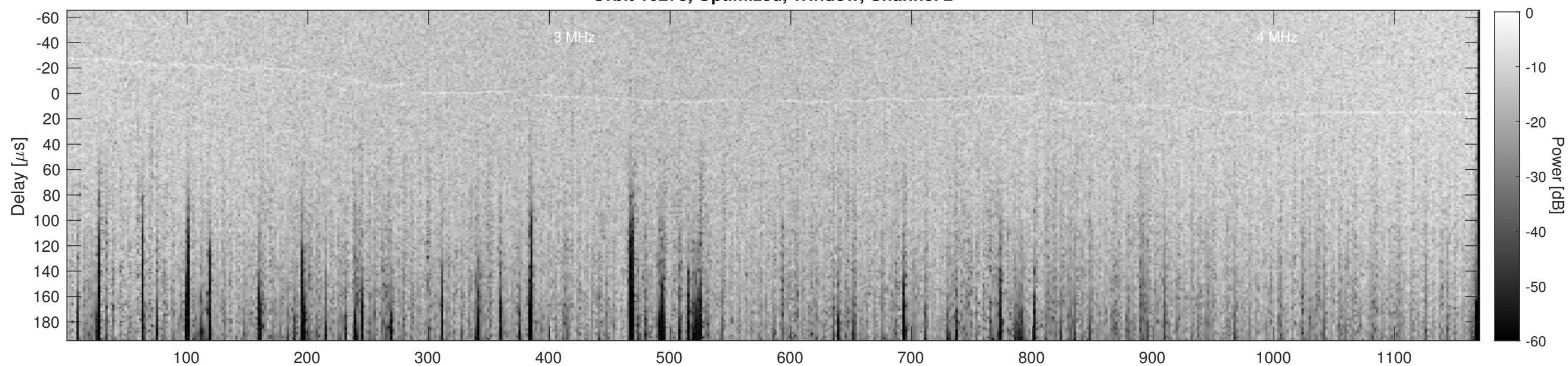
Orbit 10278, Cluttergram
