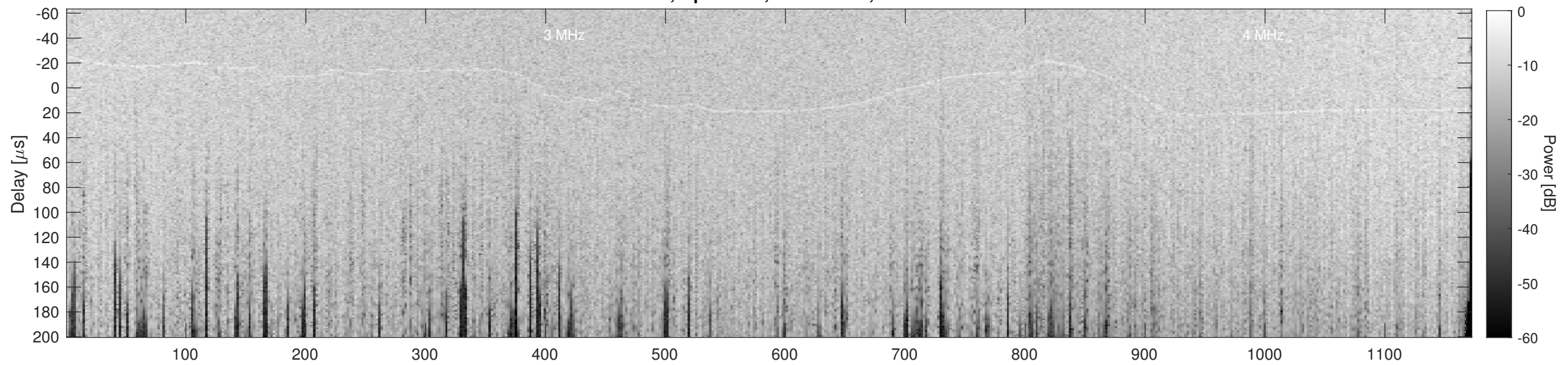
Orbit 10280, Cluttergram
