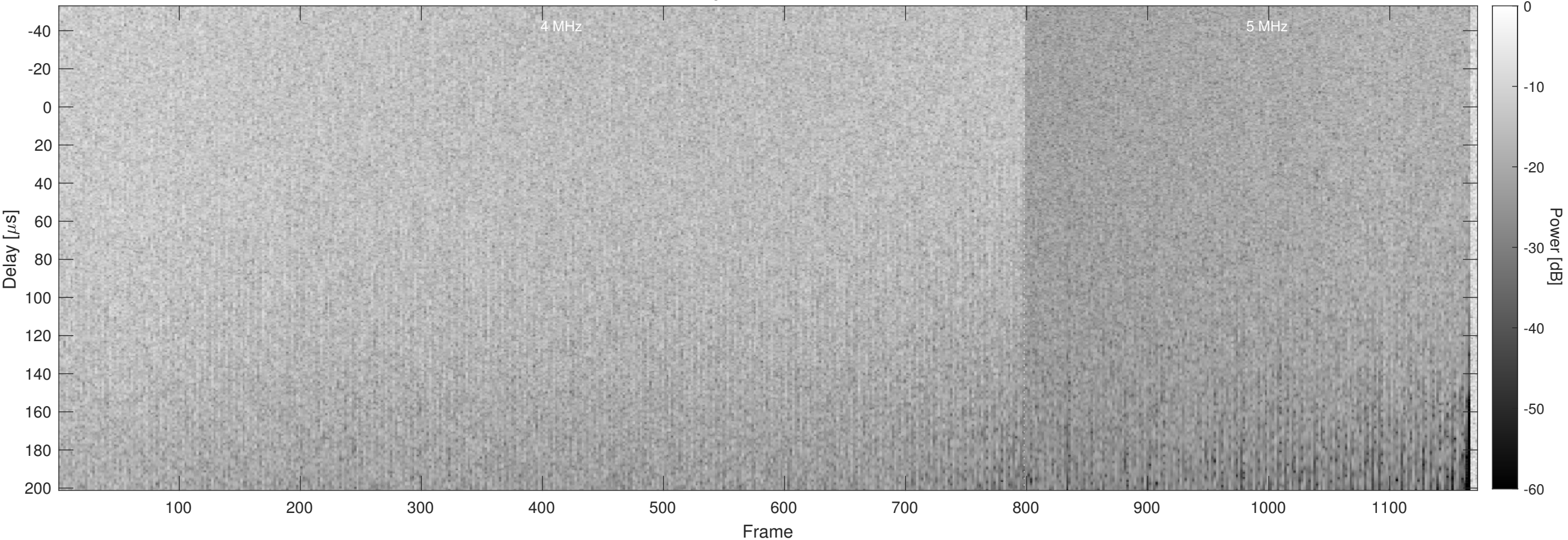
Orbit 10281, Chapman, No Window, Channel 2
