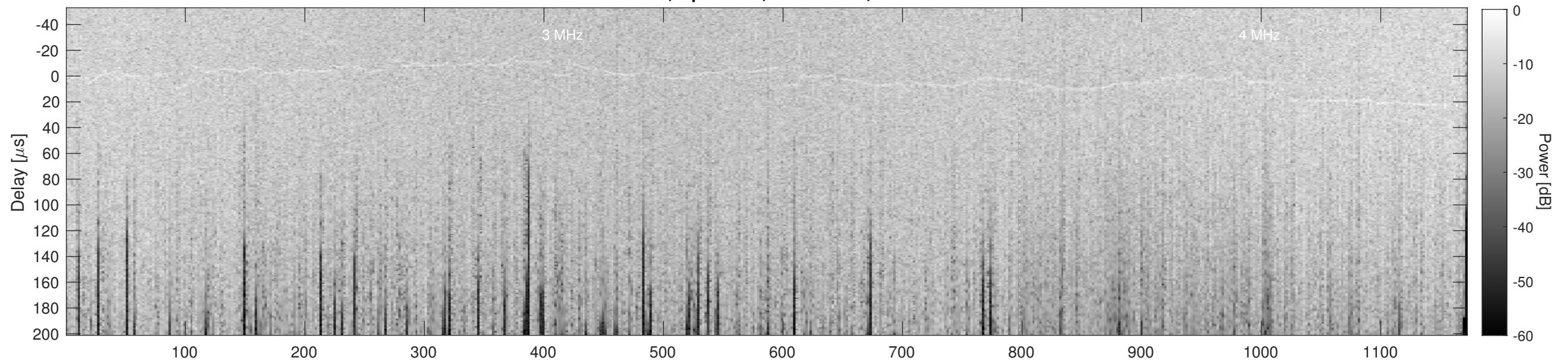
Orbit 10281, Cluttergram
