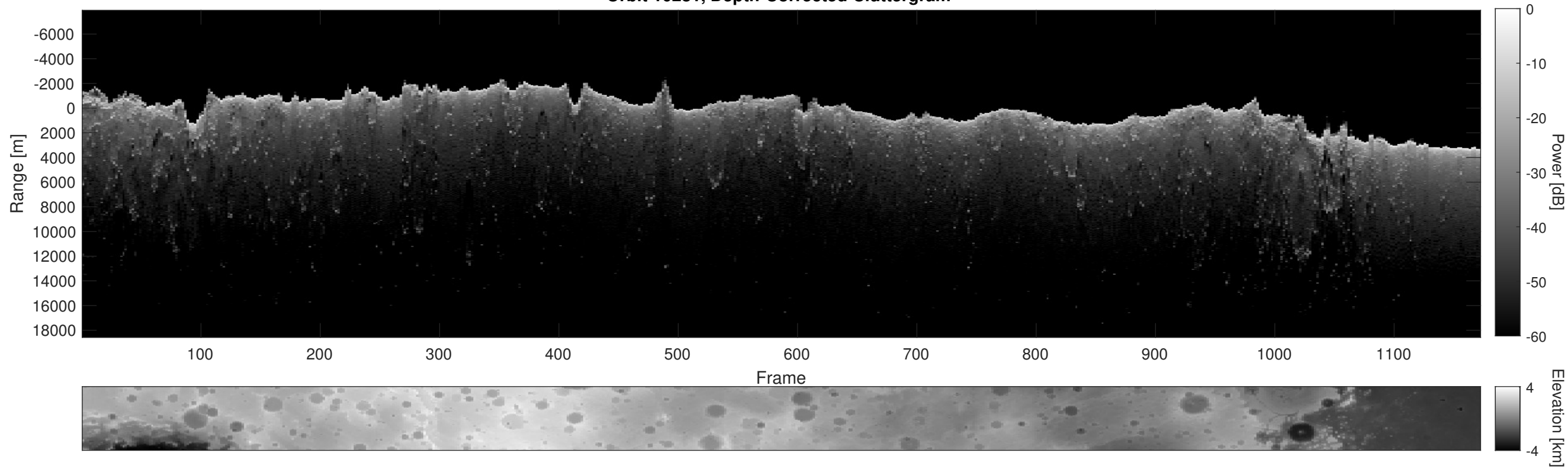
Orbit 10281, Depth-Corrected Cluttergram
