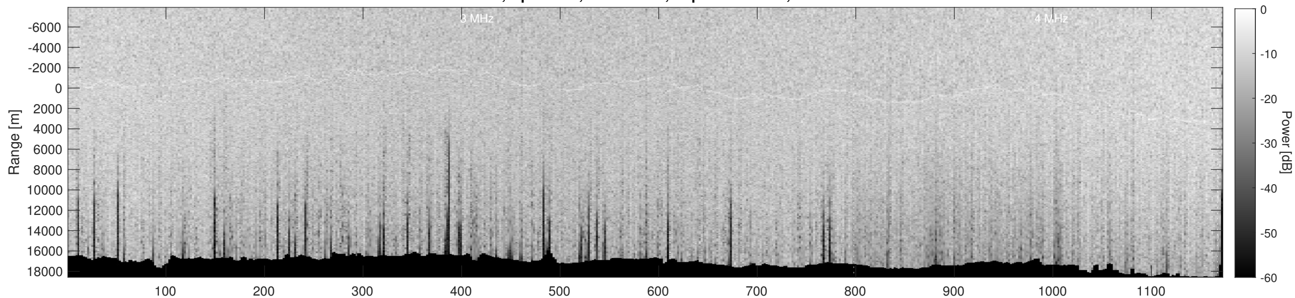
Orbit 10281, Depth-Corrected Cluttergram
