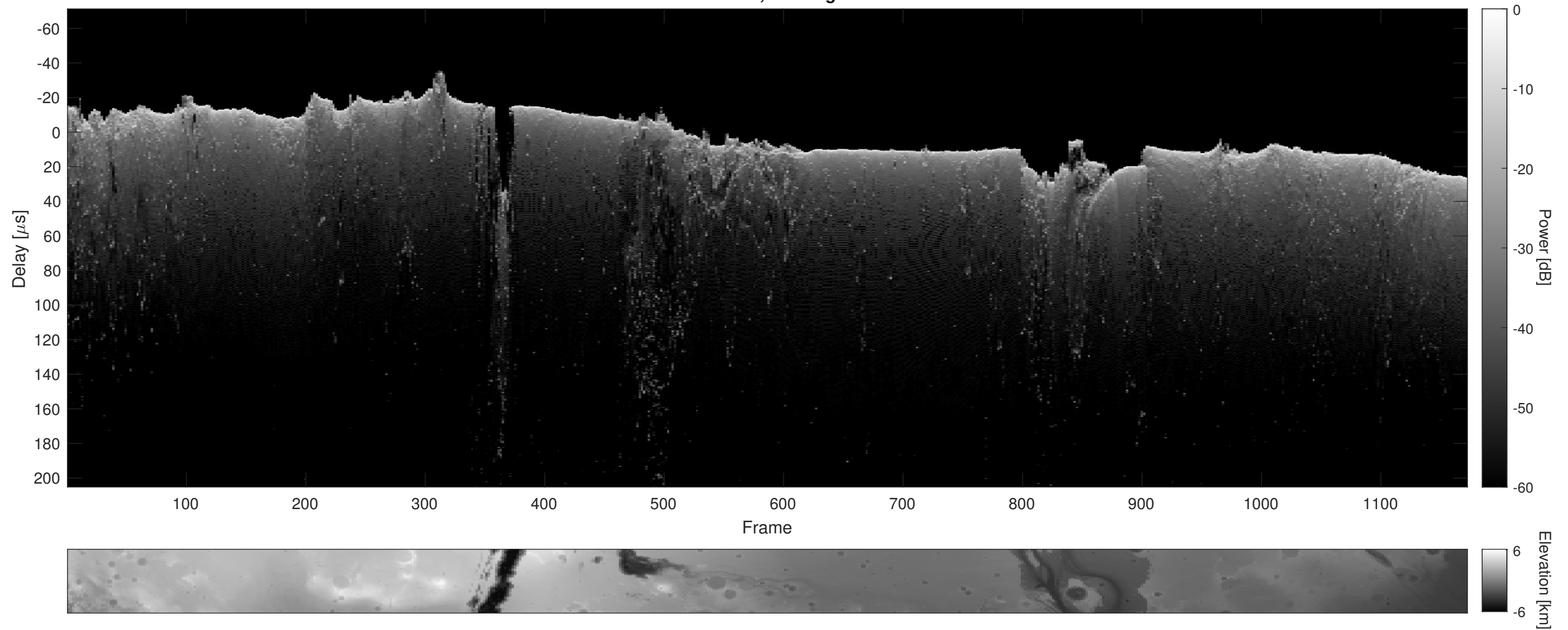
Orbit 10282, Cluttergram
