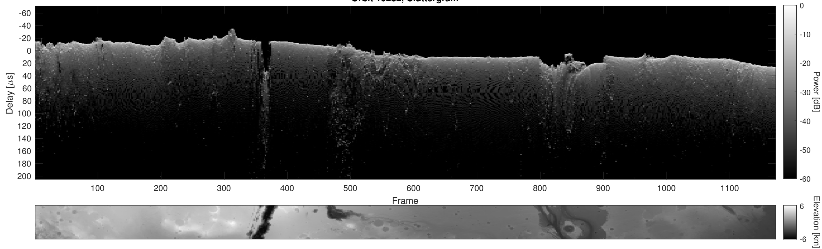
Orbit 10282, Cluttergram
