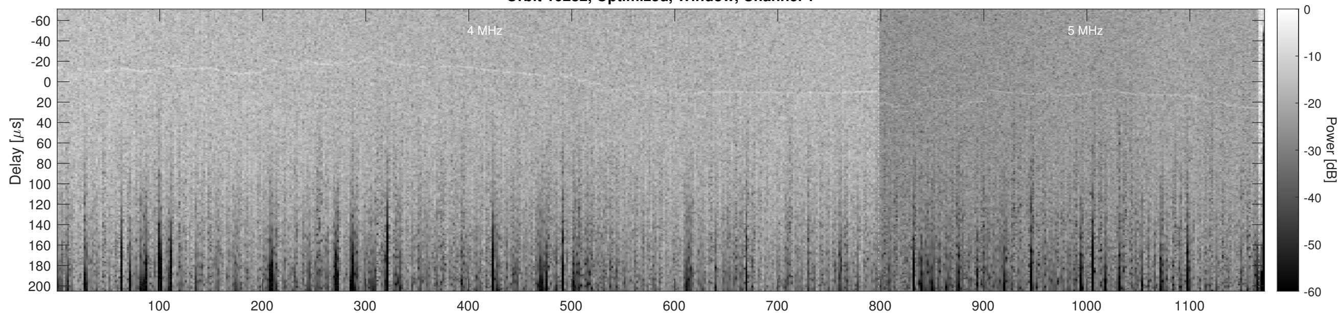
Orbit 10282, Optimized, Window, Channel 2
