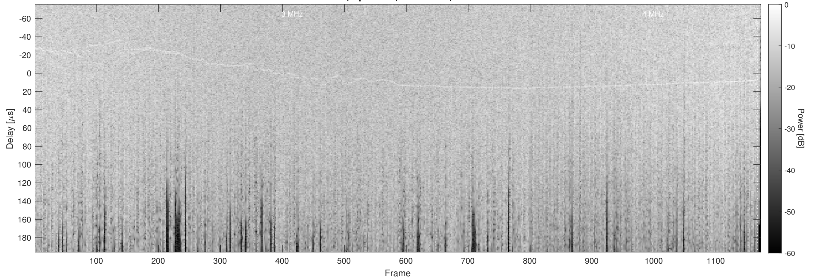
Orbit 10283, Optimized, No Window, Channel 2
