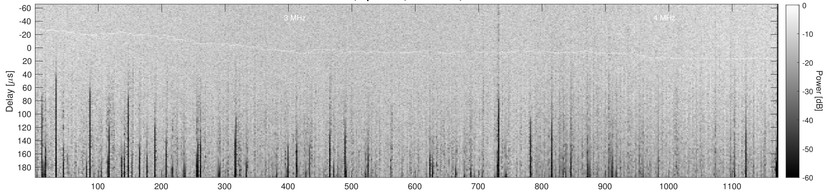
Orbit 10285, Cluttergram
