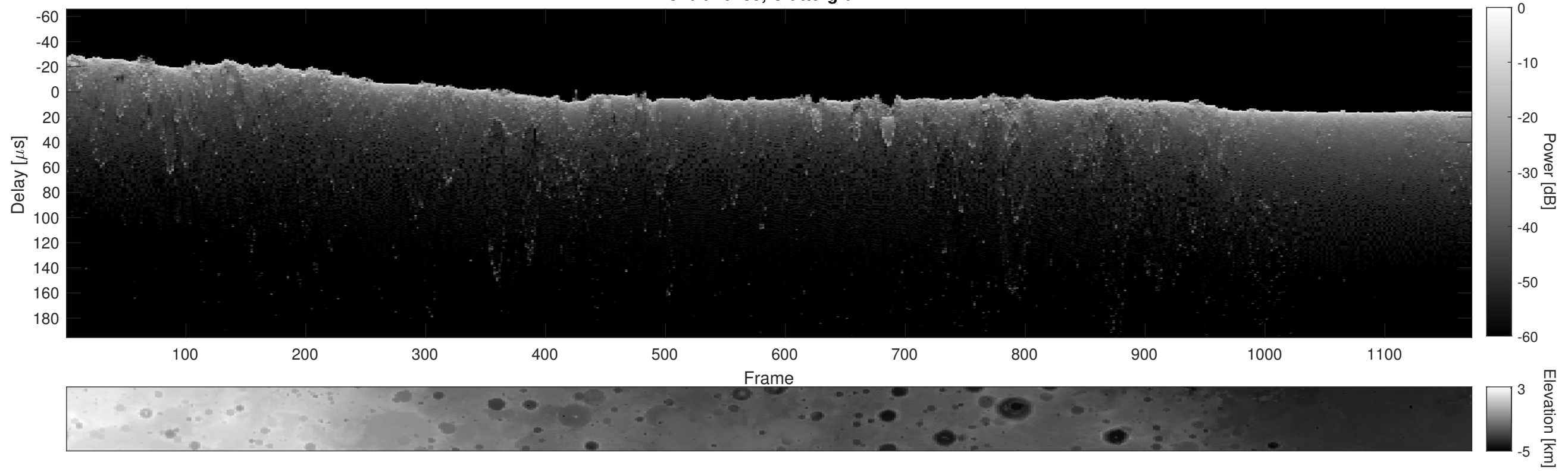
Orbit 10285, Cluttergram
