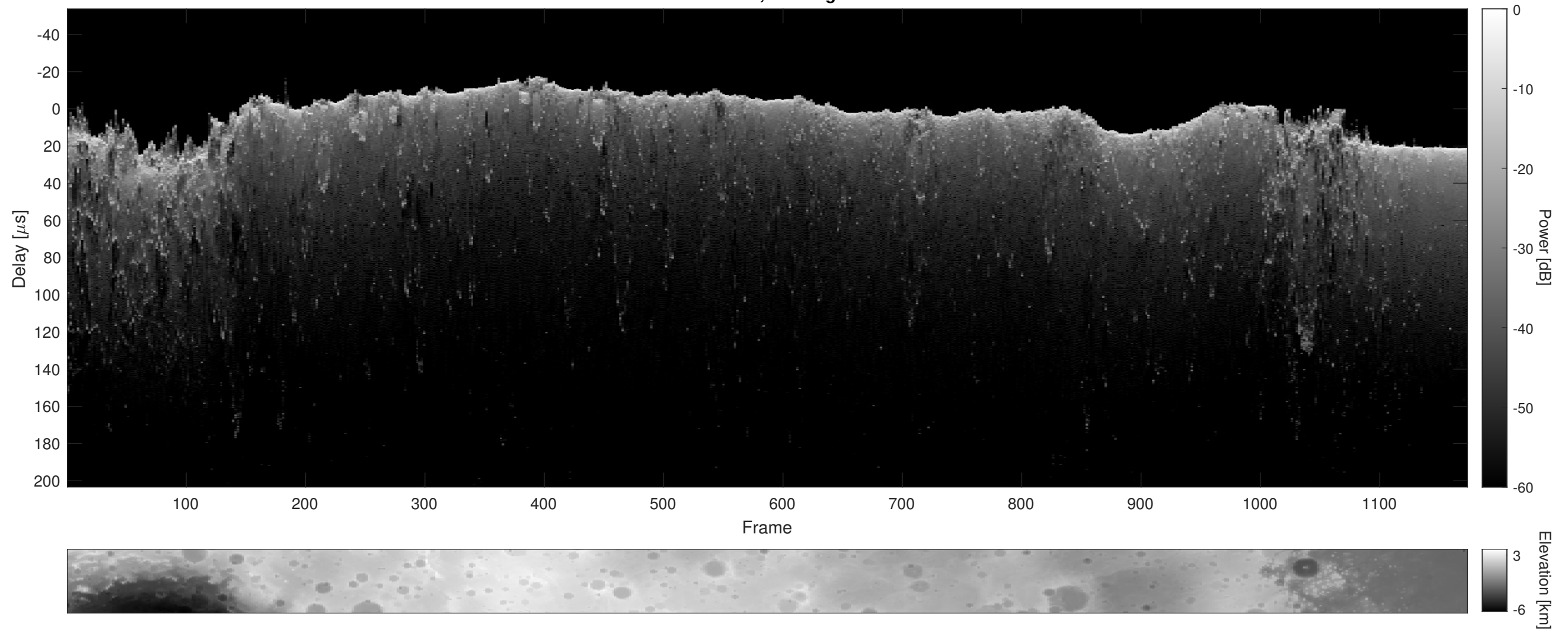
Orbit 10288, Cluttergram
