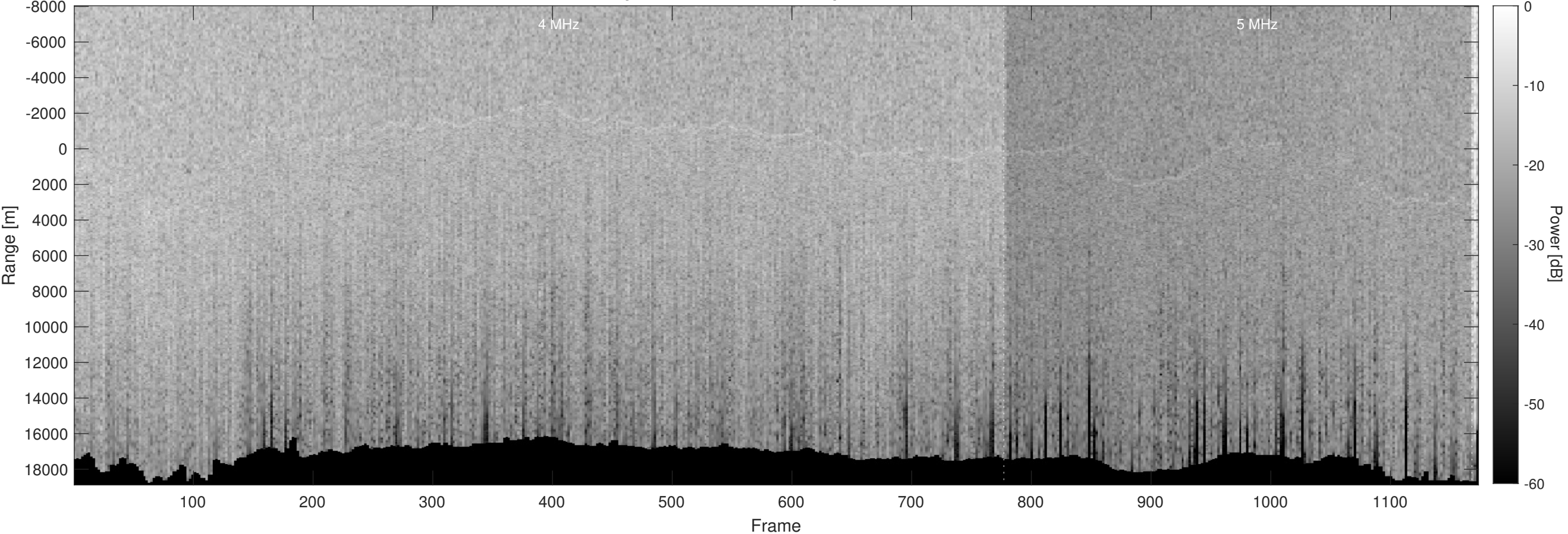
Orbit 10288, Optimized, No Window, Depth-Corrected, Channel 2
