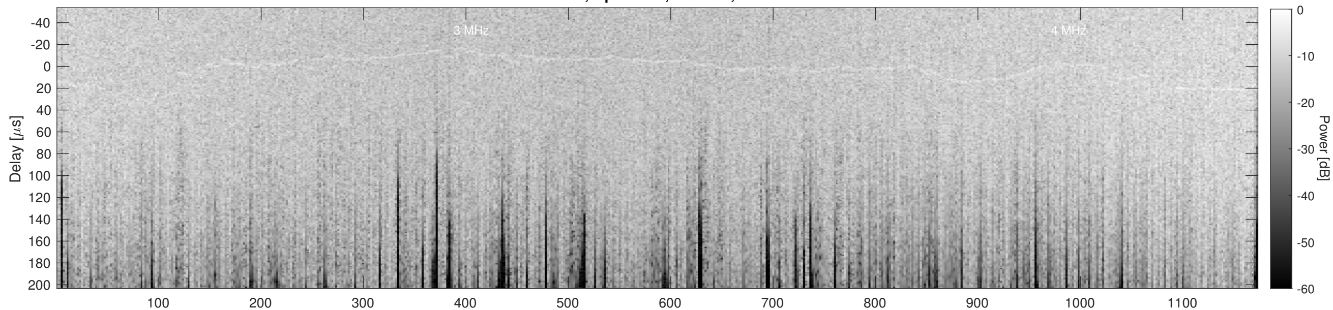
Orbit 10288, Cluttergram
