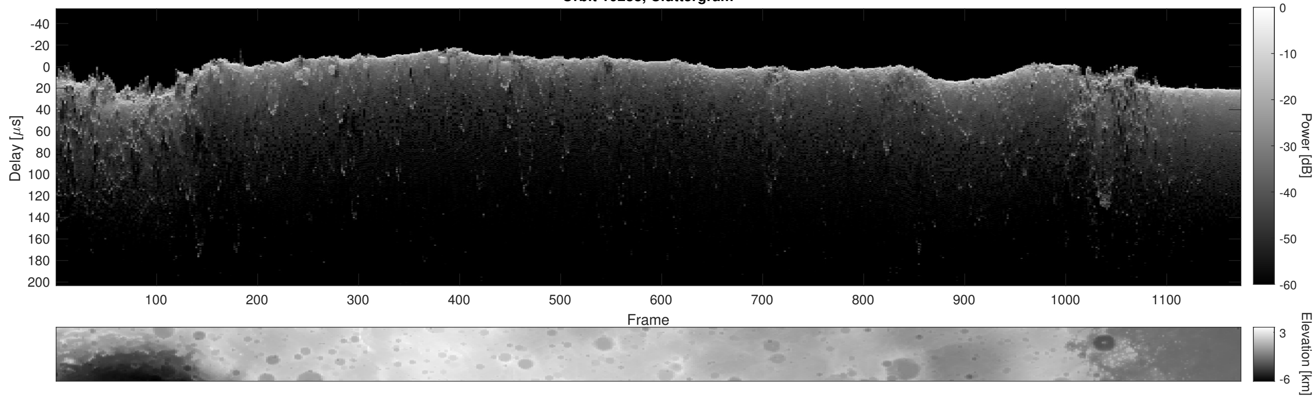
Orbit 10288, Cluttergram
