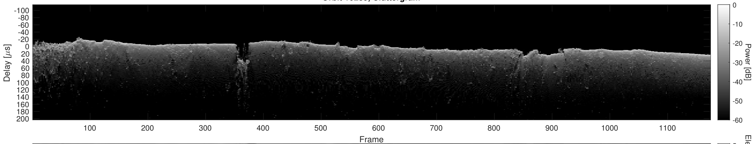
Orbit 10289, Cluttergram
