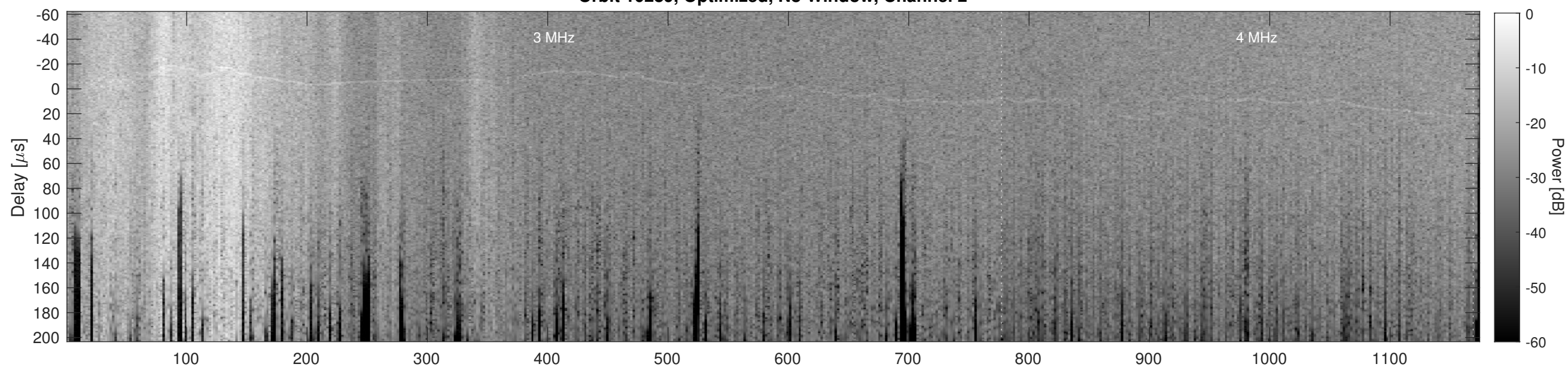
Orbit 10289, Cluttergram
