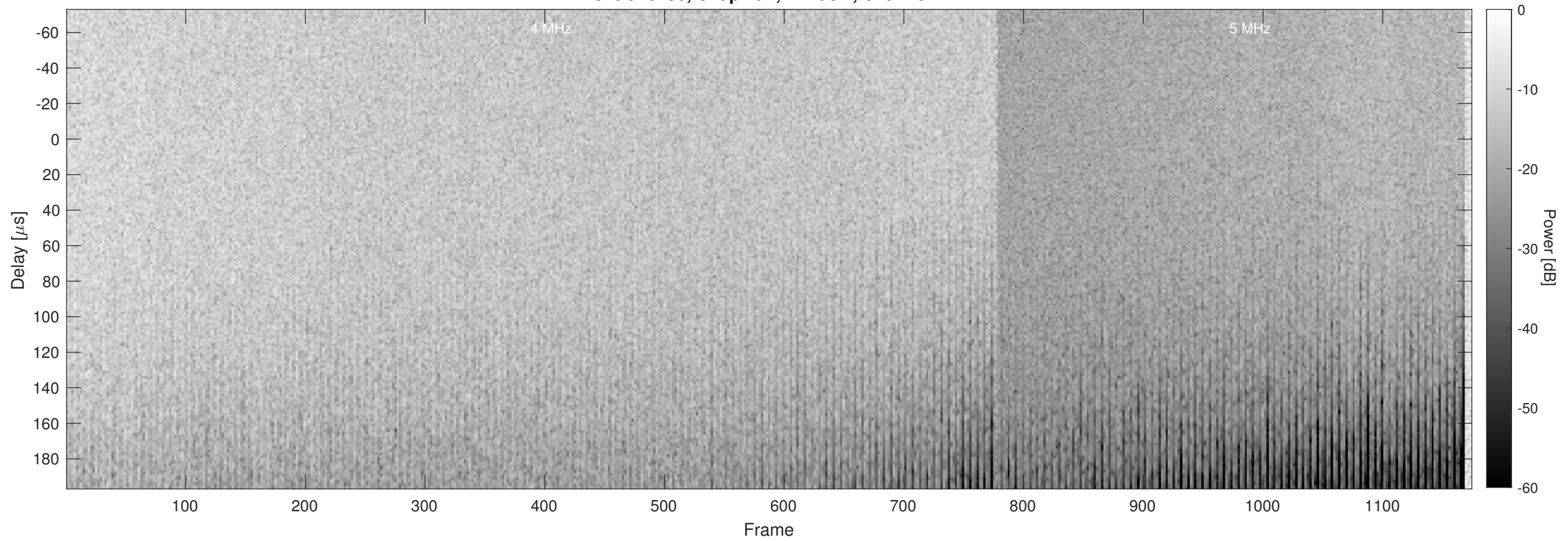
Orbit 10290, Chapman, Window, Channel 2
