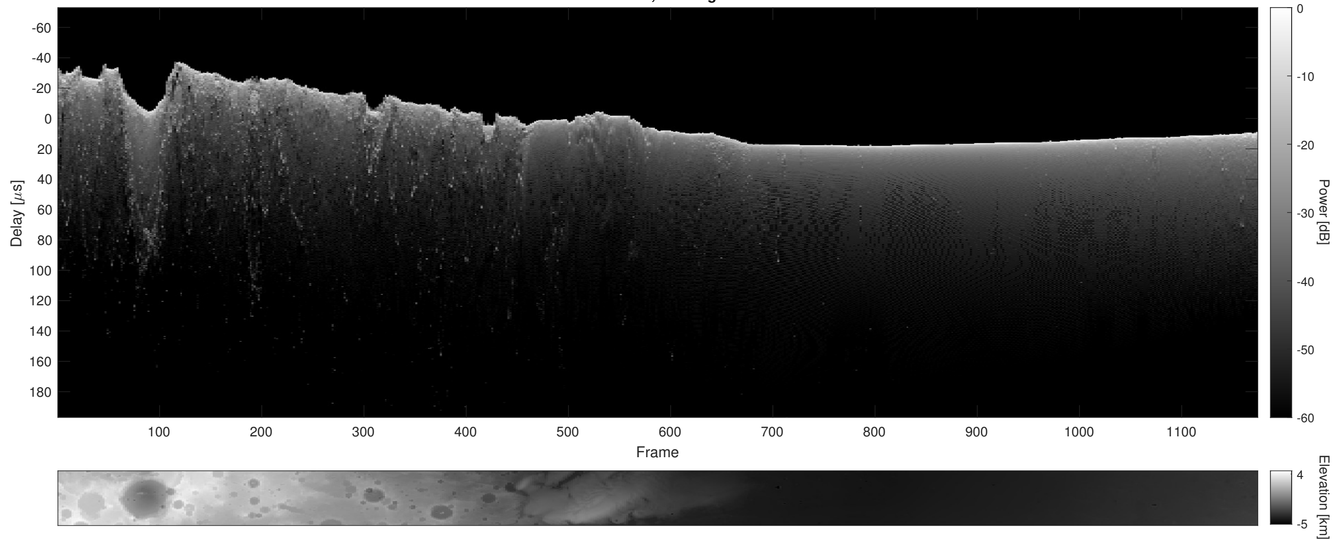
Orbit 10290, Cluttergram
