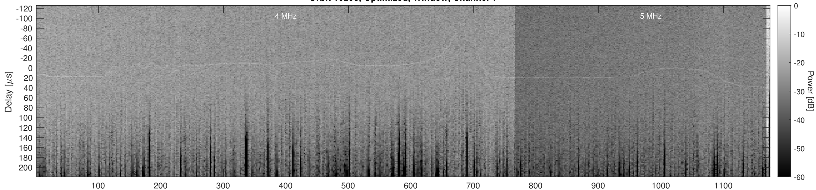
Orbit 10293, Optimized, Window, Channel 2
