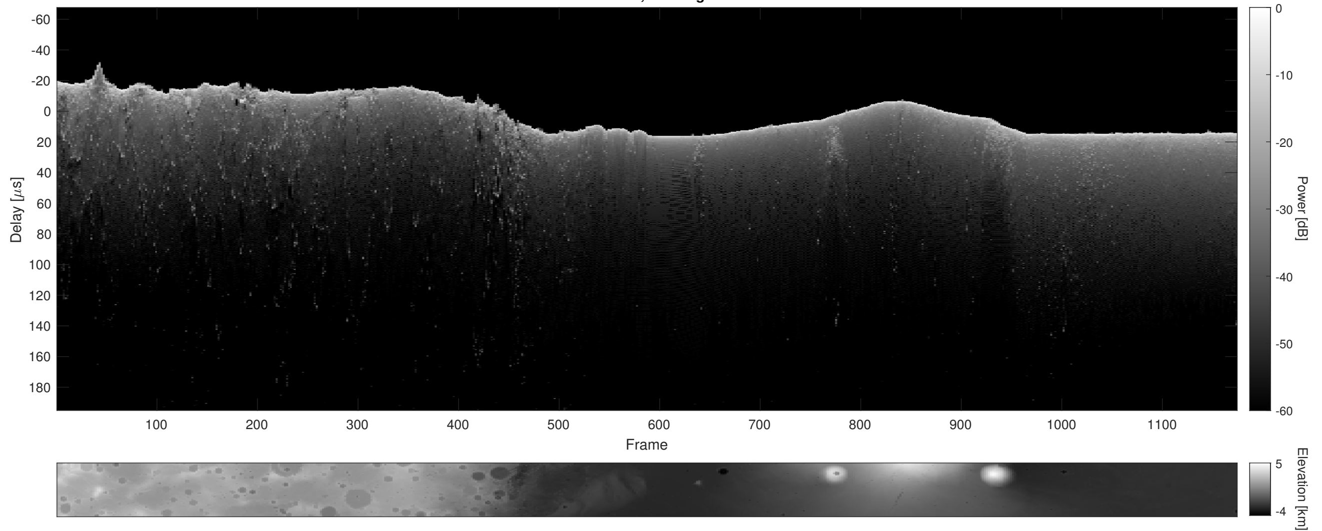
Orbit 10294, Cluttergram
