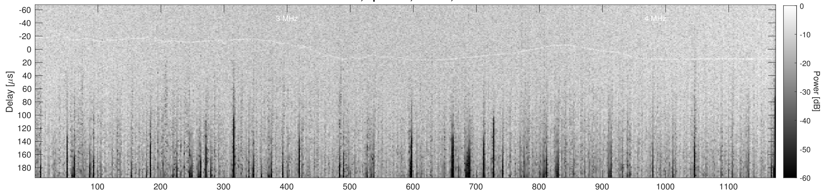
Orbit 10294, Cluttergram
