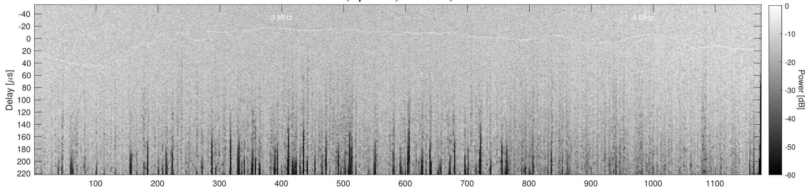
Orbit 10295, Cluttergram
