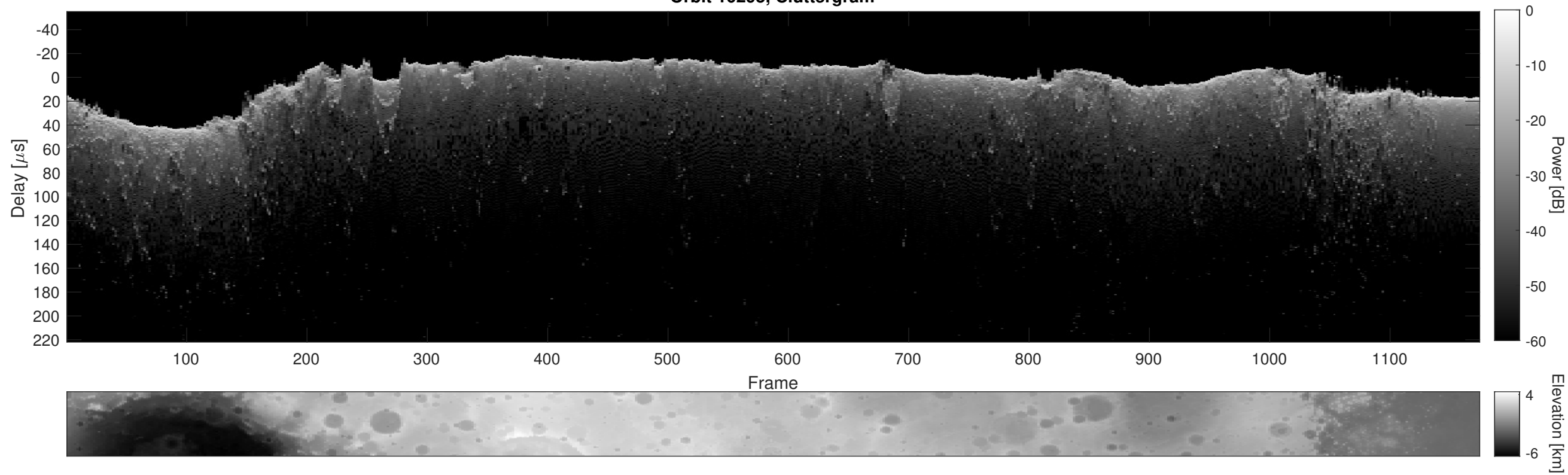
Orbit 10295, Cluttergram
