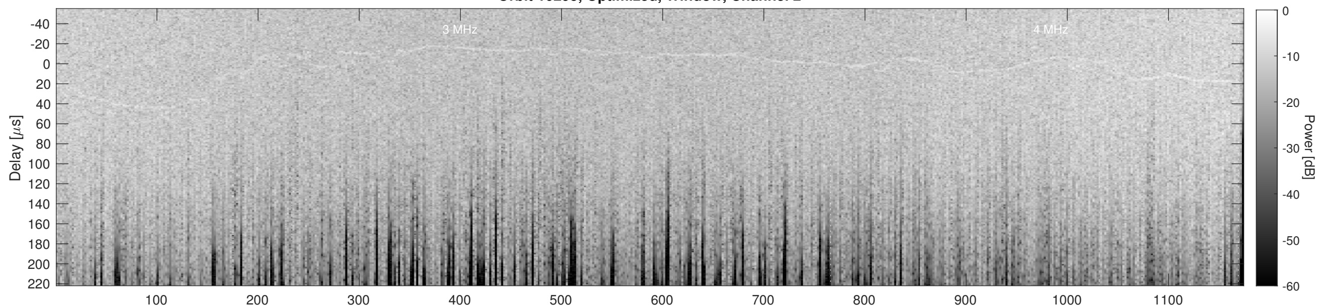
Orbit 10295, Cluttergram
