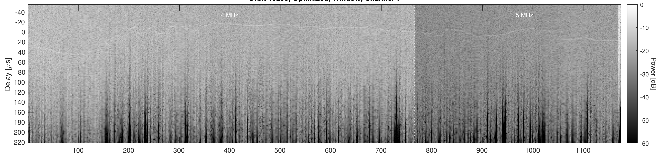
Orbit 10295, Optimized, Window, Channel 2
