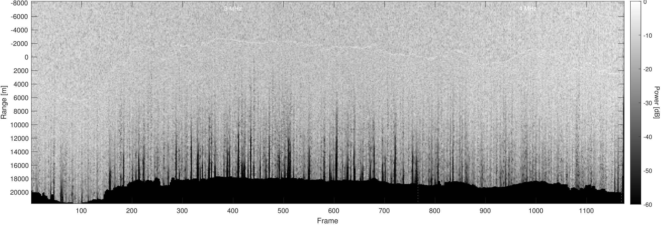
Orbit 10295, Optimized, Window, Depth-Corrected, Channel 2
