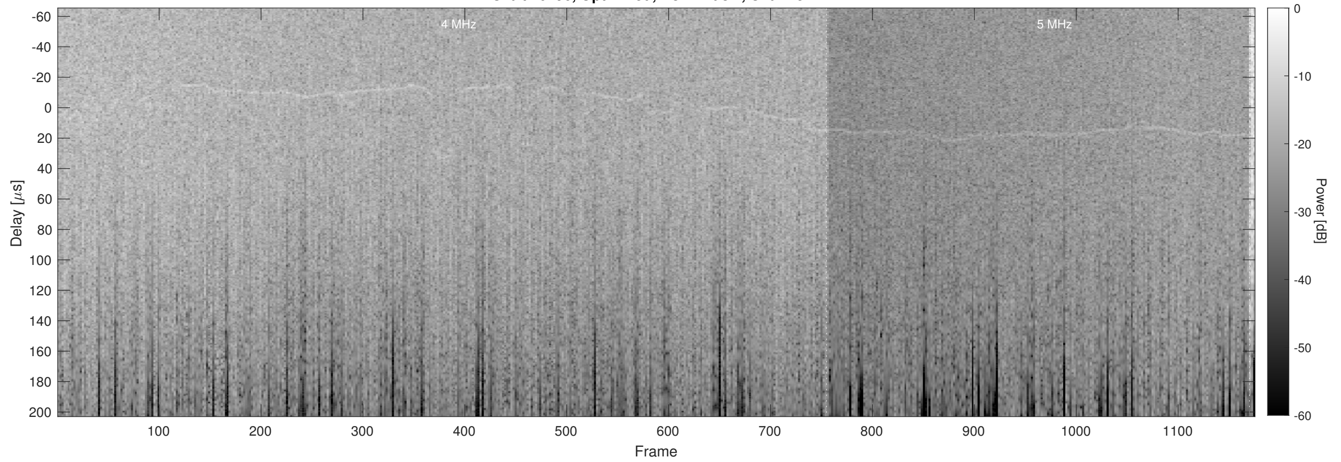
Orbit 10296, Optimized, No Window, Channel 2
