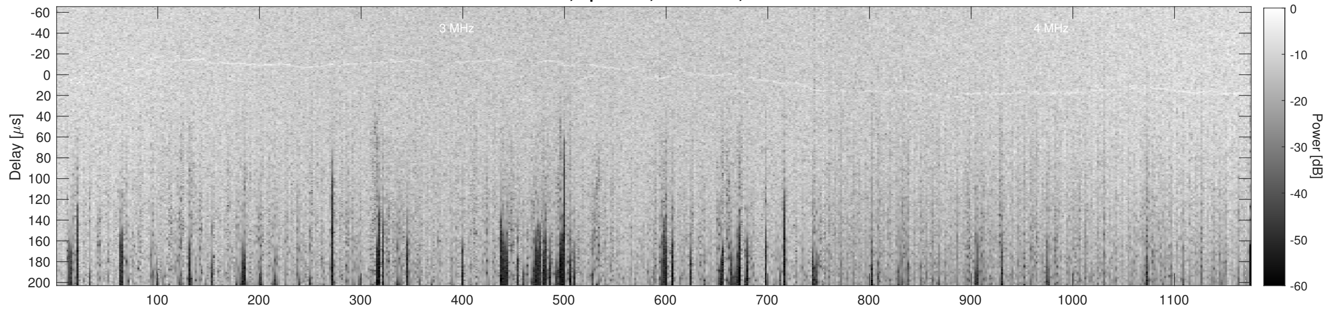
Orbit 10296, Cluttergram
