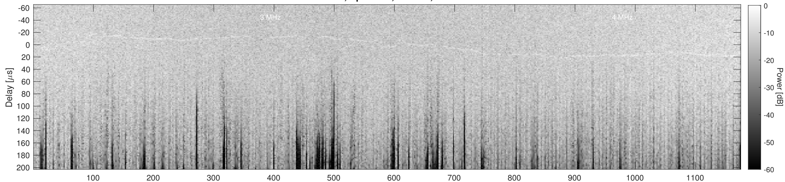
Orbit 10296, Cluttergram
